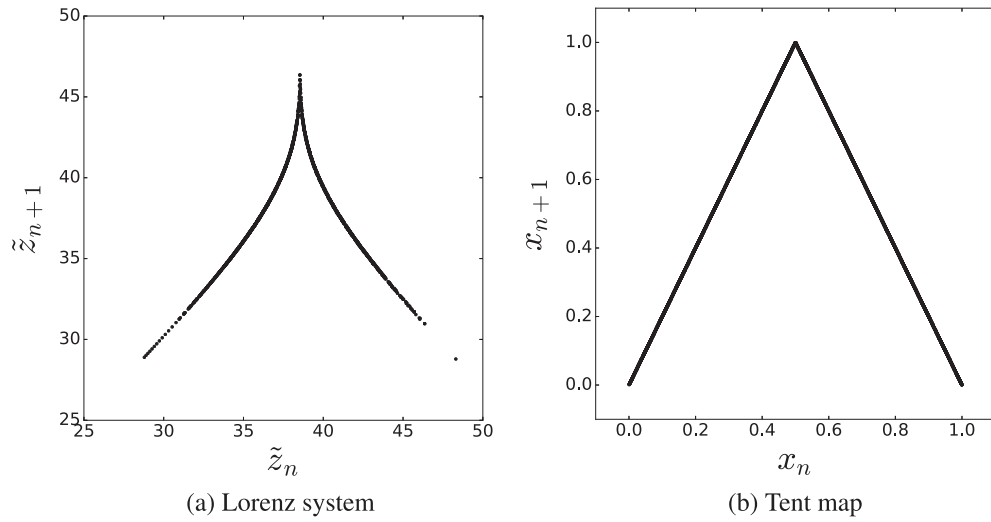
Figure 1. Similarity between Poincaré map of Lorenz system and the tent map.
