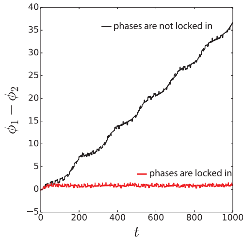
Figure 14. Illustration of phase synchronisation for two coupled slightly different and chaotic systems ( f_1 \neq f_2 ). The evolution of the phase differences between the systems for two different coupling constants \alpha < \alpha_c and \alpha > \alpha_c .
