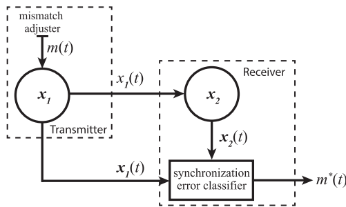
Figure 18. A secure communication scheme: hiding a digital message on a chaotic signal. Changing a parameter of transmitter causes different level of synchronisation errors between the transmitter and the receiver. The amplitude of the error E brings the message out.
