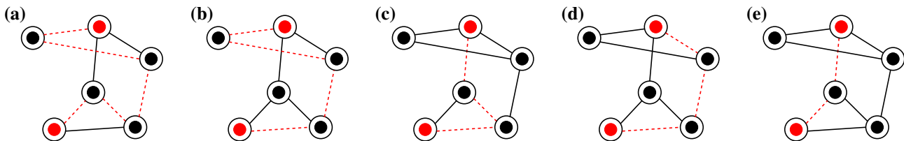
Figure 30. Visualisation of paths (red dashed) between two selected nodes (red) in a network: path length of (a) is five, (b) is four, (c) and (d) are three and (e) is two. Therefore the shortest path length for these two red nodes is two.
