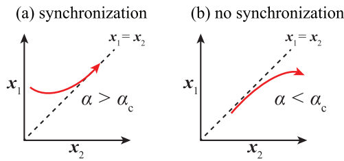
Figure 13. Illustration of complete synchronisation. (a) If the coupling strength is large enough ( \alpha > \alpha_c ), the systems converge to invariant synchronisation manifold ( x_1 = x_2 ), (b) otherwise ( \alpha < \alpha_c ), they diverge hence no synchronisation.
