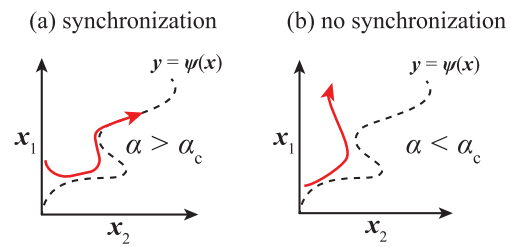
Figure 15. Illustration of generalised synchronisation. If the coupling strength is large enough, a functional relationship ( y = \psi(x) ) exhibits between the dynamical variables x_1 and x_2 . (a) If \alpha > \alpha_c , the generalised synchronisation is observed (b) otherwise \alpha < \alpha_c , there is no generalised synchronisation.
