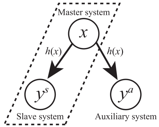
Figure 9. Scheme of the auxiliary system approach for the generalised synchronisation. Originally we only have the system in the dashed line box which is master–slave system as in Section 2.2.1. Then we add an auxiliary (helper) system y^a . If there is CS between y^s and y^a , then the GS occurs between x and y^{a,s} .
