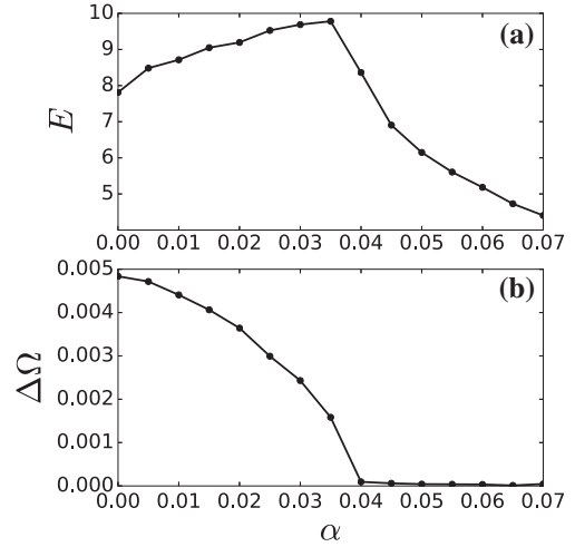
Figure 8. For a weak coupling constant: Although there is no synchrony for the difference of the amplitudes Equation (15) (top panel), there is a tendency towards to phase synchronisation while the coupling constant \alpha increases Equation (24) (bottom panel). The synchronisation error E and frequency mismatch \Delta\Omega were averaged over 300 realisations. Each realisation is simulated by a fourth-order Runge–Kutta scheme for 2000 s with 0.01 time step.
