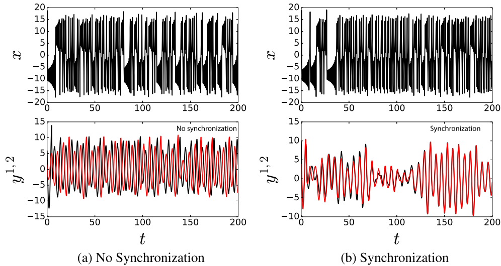
Figure 11. Two simulations for the generalised coupling scheme: a Lorenz system x drives two Rössler systems y^{s,a} . The critical transition coupling is \alpha_c \approx 0.12 . (a) For the coupling constant \alpha = 0.06 , there is no synchronisation since \alpha < \alpha_c (b) for \alpha = 0.2 synchronisation is obtained since \alpha > \alpha_c .
