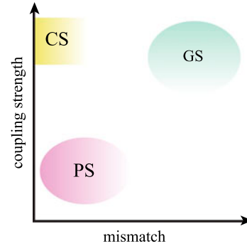
Figure 12. Diagram of synchronisation types for diffusively coupled systems. The horizontal axis depicts the mismatch between the isolated dynamics ( f_1 and f_2 ) and the vertical axis the coupling constant. The diagram shows the typical balance between mismatch and coupling strength and to achieve a certain kind of synchronisation. Complete synchronisation (CS) occurs for identical chaotic systems ( f_1 = f_2 ) and large enough coupling strengths. Phase synchronisation (PS) is observed between slightly different systems for small coupling strengths. Generalised synchronisation (GS) is a result of master–slave system and can occur for large mismatch parameters or even between distinct systems when the coupling strength large enough.
