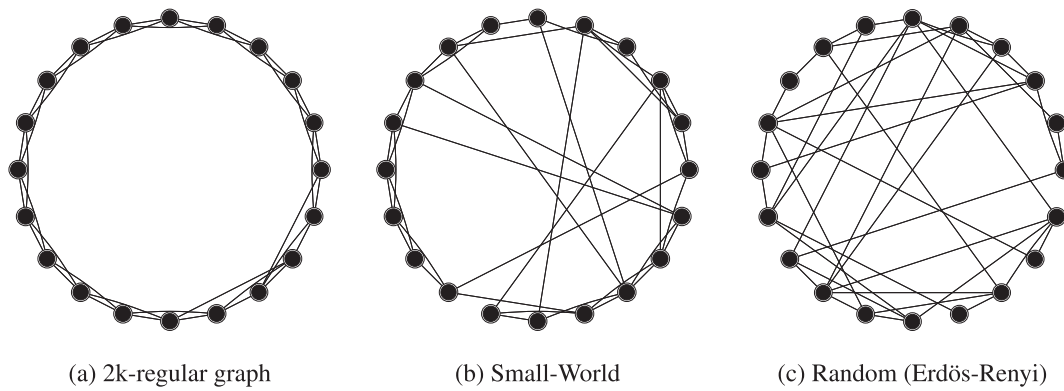
Figure 32. Watts–Strogatz random network approach.
