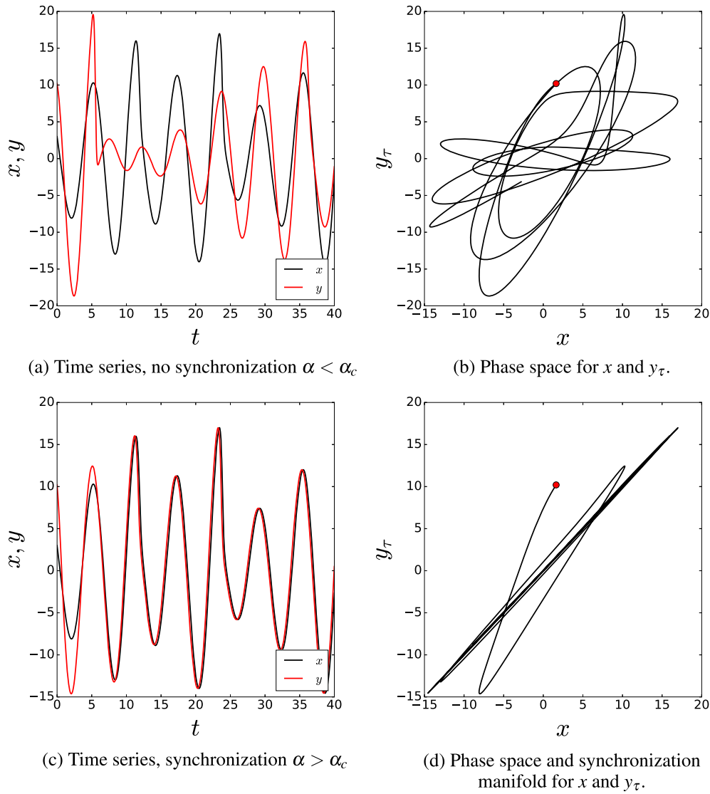
Figure 27. Anticipating synchronisation does not obtain for (\alpha < \alpha_c) , otherwise (\alpha > \alpha_c) the AS exhibits. For this illustration the delay is selected as \tau = 0.2 . (a) time series of the systems where \alpha < \alpha_c and (b) phase space. (c) time series of the systems where \alpha > \alpha_c and (d) phase space and synchronisation manifold of the system. The red circle is the initial condition for the trajectory of (x, y_\tau) .
