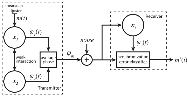
Figure 20. A secure communication scheme by phase synchronisation: hiding a digital message on a chaotic signal.
