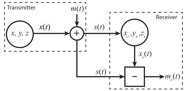
Figure 16. Illustration of the message masking on bearing signal scheme. Transmitter generates a chaotic signal x(t) and add the message m(t) on it. This combined two signals s(t) = x(t) + m(t) is sent to the receiver and both systems synchronise. Discarding the synced signal x_r from the s , the message m_r \sim m is restored.
