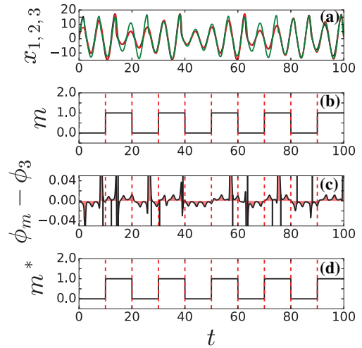
Figure 21. An illustration for the secure communication by phase synchronisation: hiding a digital message on a chaotic signal.
