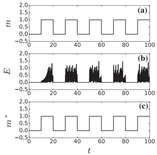
Figure 19. Manipulating the parameter of a transmitter allows digital secure communication. In this application 10 time units are used for a single digit. (a) Digital message (0101010101), (b) the synchronisation error and (c) restored message.
