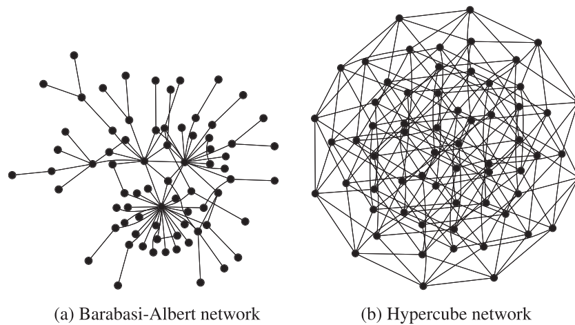
Figure 33. Some examples of complex networks.
