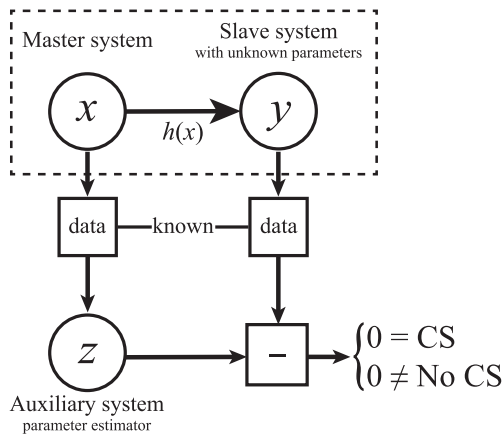
Figure 22. Only two data-sets are known from a master–slave system, into the dashed rectangle, without any info about the parameters. An auxiliary system is driven by the data from the master and measures the amplitude difference between the auxiliary and the data from the slave system. If the difference is 0, then there is a CS that means the parameters of the slave and the auxiliary are identical.
