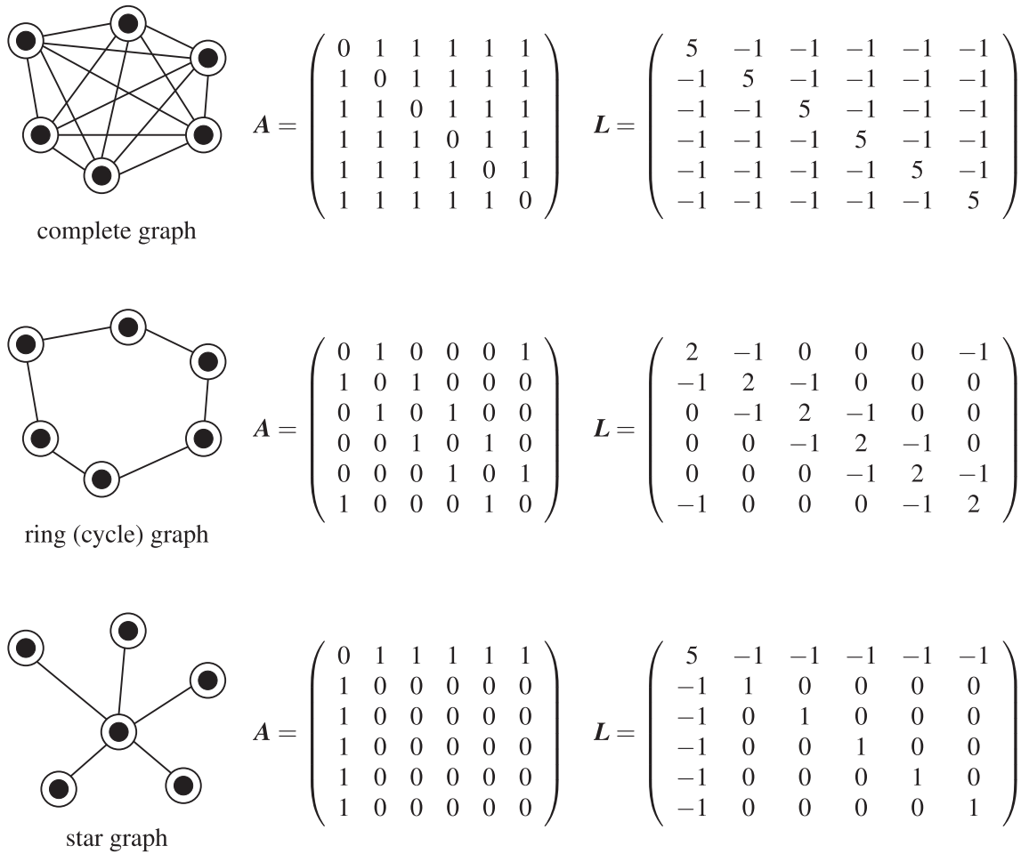
Figure 31. Various network examples with six nodes. Their adjacency A and Laplacian L matrices.
