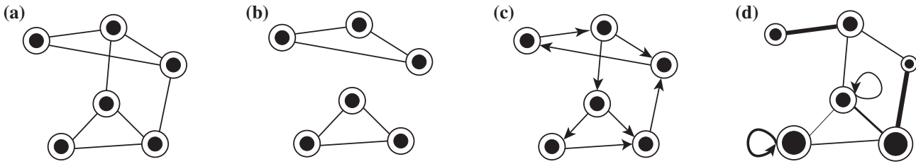
Figure 29. Visualisation of network types: (a) an unweighted simple network, (b) a disconnected network, (c) a directed network, (d) a weighted network with self-loops.
