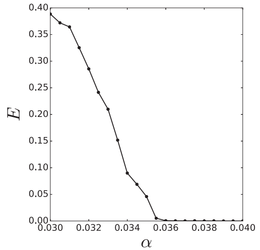
Figure 4. The synchronisation diagram of two coupled Rössler systems with the coupling function \mathbf{H} = \mathbf{I} . The theoretical critical coupling constant \alpha_c \approx 0.0355 indeed corresponds to the numerically observed one. The synchronisation error E was averaged over 300 realisations. Each realisation is simulated by a fourth-order Runge–Kutta scheme for 2000 s with 0.01 time step.
