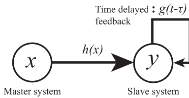
Figure 26. Scheme of anticipating synchronisation without memory in the driver systems.
