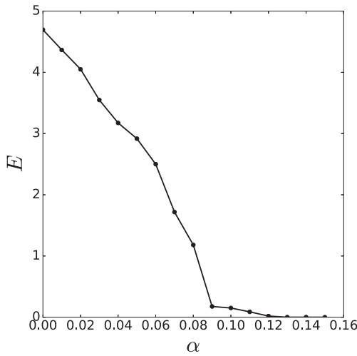
Figure 10. Generalised synchronisation: averaged over 300 realisations, time = 4000 and time step = 0.01.
