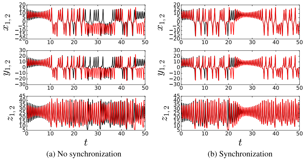
Figure 2. Comparison of trajectories of two initial conditions for the system of two coupled Lorenz systems. The critical transition coupling is \alpha_c \approx 0.453 for the classical parameters. The initial conditions are selected as (x_1, y_1, z_1) = (3, 10, 15) and (x_2, y_2, z_2) = (10, 15, 25) . (a) When \alpha = 0.4 < \alpha_c , there is no synchronisation. (b) If \alpha = 0.5 > \alpha_c one observes synchronisation of trajectories.
