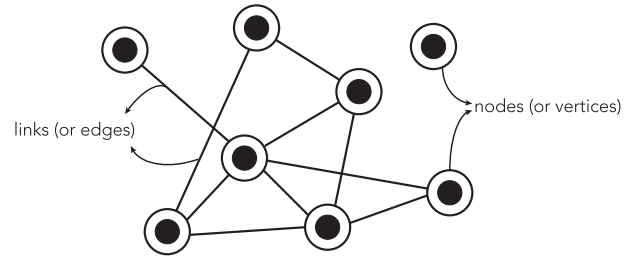
Figure 28. A network visualisation with eight nodes and ten links.
