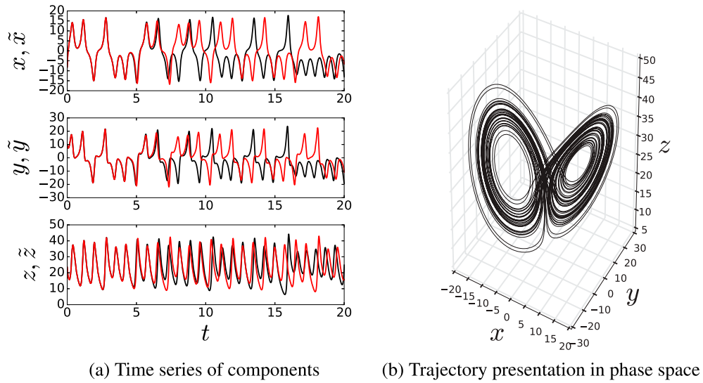
Figure 1. Illustration of the chaotic dynamics of the Lorenz system (14) with parameter values \sigma = 10 , \rho = 28 and \beta = 8/3 . (a) Two simulations for the Lorenz system starting from two slightly different initial conditions (x, y, z) = (-10, 10, 25) and (\tilde{x}, \tilde{y}, \tilde{z}) = (-10.01, 10, 25) . The Lorenz attractor has a positive Lyapunov exponent and the trajectories diverge from each other. (b) Representation of the trajectory of (x, y, z) = (-10, 10, 25) in the phase space. The shape of the attractor resembles a butterfly.
