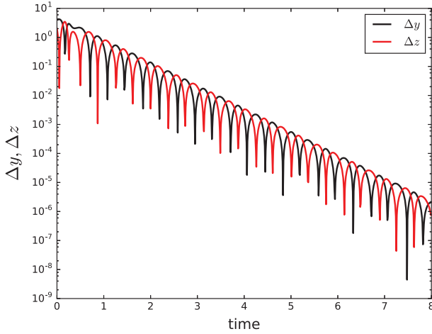
Figure 6. Simulation of master–slave type of coupling.
