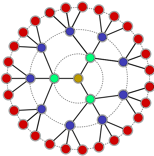
Figure 36. Bethe lattice graph: an example of symmetries in network structure. Nodes in the same level of the Bethe graph are exactly symmetric to each other. Therefore same colour nodes constitute a cluster.
