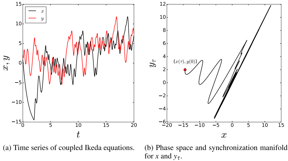
Figure 25. Anticipating chaotic synchronisation. In the beginning, the systems are not in harmony. After a transient time both systems are getting into a time-delay \tau synchronisation. For this illustration \tau = 2 . (a) time series of the systems (b) phase space and synchronisation manifold of the system. The red circle is the initial condition for the trajectory of (x, y_\tau) .
