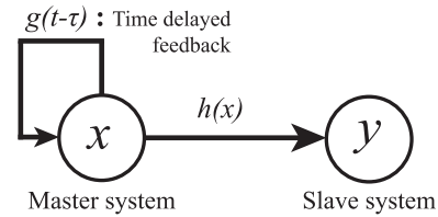
Figure 24. Scheme of anticipating synchronisation with memory in the driver systems.
