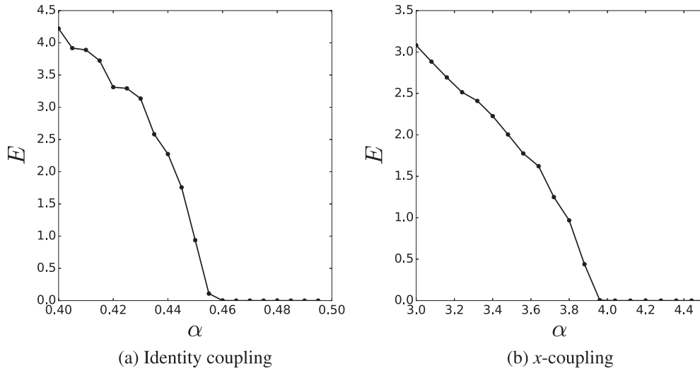
Figure 3. Synchronisation diagram of two coupled Lorenz systems, (a) with coupling matrix \mathbf{H} = \mathbf{I} and (b) with coupling matrix \mathbf{H} as in Equation (16). When \mathbf{H} = \mathbf{I} , the observed critical coupling constant corresponds to the theoretically derived value \alpha_c \sim 0.453 . With coupling matrix (16), synchronisation is observed to set in for coupling strengths larger than \sim 3.75 . The synchronisation error E was averaged over 300 realisations. Each realisation is simulated by a fourth-order Runge–Kutta scheme for 2000 s with 0.01 time step.
