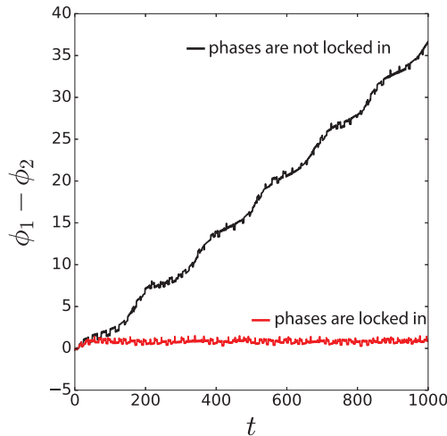
Figure 14. Illustration of phase synchronisation for two coupled slightly different and chaotic systems ( f_1 \neq f_2 ). The evolution of the phase differences between the systems for two different coupling constants \alpha < \alpha_c and \alpha > \alpha_c .
