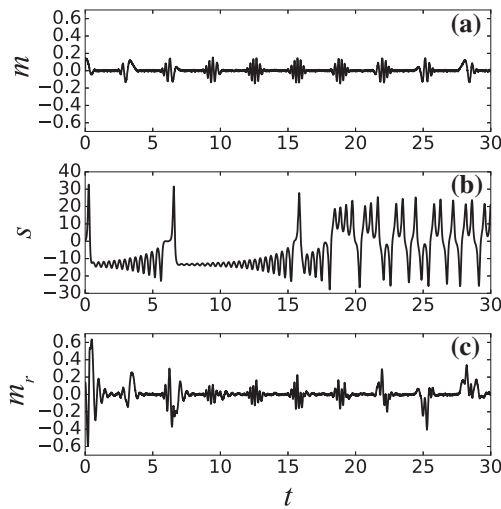
Figure 17. The masking an analog message on bearing chaotic signal. (a) The low-amplitude message, (b) the message embedded into high-amplitude chaotic signal and (c) restored message from the transmitted signal.
