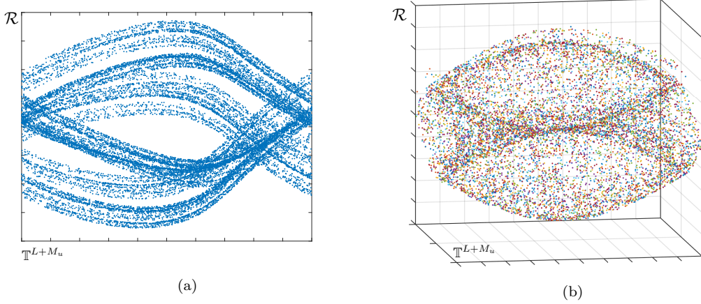
Figure 5: Approximate 2D and 3D representations of one component of the attractor of F_\varepsilon .
