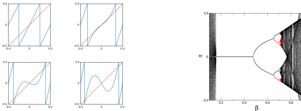
Figure 2: On the left the graphs of T_\beta for \beta = 0, 0.2, 0.4, 0.6 . On the right the bifurcation diagram for the reduced dynamics of hubs. We considered the identification \mathbb{T} = [-1/2, 1/2]/\sim . We obtained the diagram numerically. To build the bifurcation diagram we reported a segment of a typical orbit of length 10^3 , for a collection of values of the parameter \beta .
