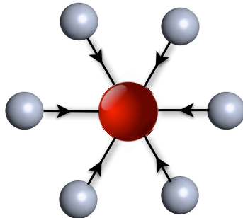
Figure 4: Star network with only incoming arrows.
