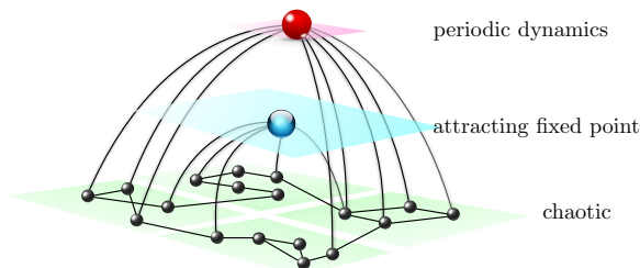
Figure 1: The dynamics across connectivity layers change depending on the connectivity of the hubs. We will exhibit an example where the hubs with the highest number of connections (in red, at the top) have periodic dynamics. In the second connectivity layer, where hubs have half of the number of connection (in blue, in the middle), the dynamics sits around a fixed point. In the bottom layer of poorly connected nodes the dynamics is chaotic. (Only one hub has been drawn on the top two layers for clarity of the picture).
