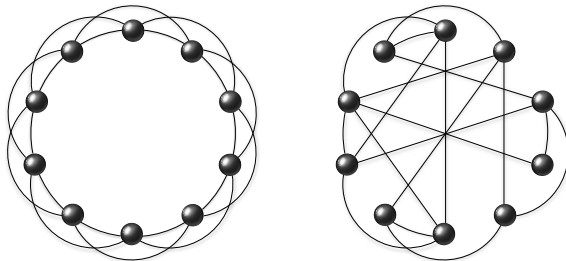
Figure 7: On the left panel we present a regular network where every nodes connects to its 2 left and 2 right nearest neighbors. Such networks shows poor synchronization properties in the large N limit if K \ll N as shown in Eq. (??). On the right panel, we depict a random (Erdős-Rényi) network where every connection is a Bernoulli random variable with success probability p = 0.3 . Such random networks tend to be homogeneous (nodes have pN connections) and they exhibit excellent synchronization properties.
