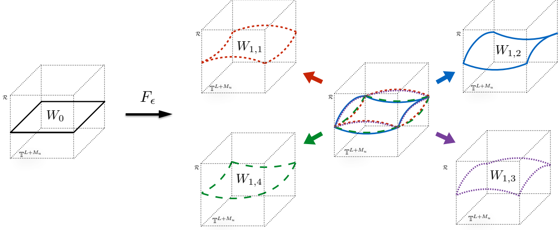
Figure 6: The admissible manifold W_0 is mapped under F_\varepsilon to the union of sub manifolds W_{1,1} , W_{1,2} , W_{1,3} , and W_{1,4} .
