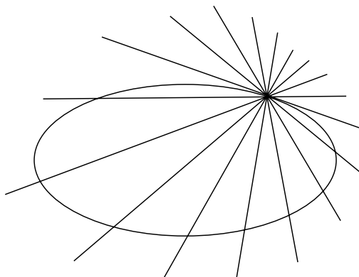
Fig. 15.18. The tangent line to the ellipse at P is the only straight line through P that has no point inside the ellipse.
