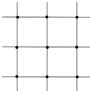
Fig. 15.27. Square network.
