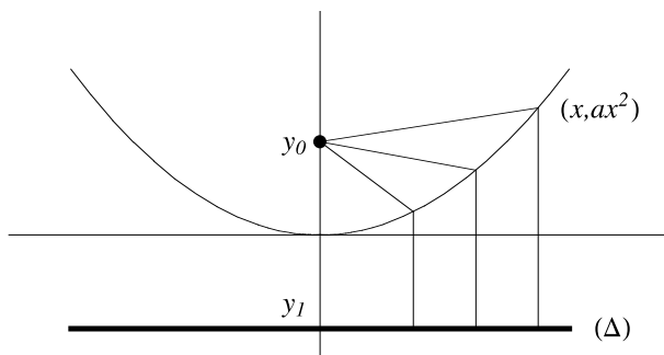
Fig. 15.7. The geometric definition of a parabola.
