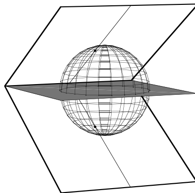
(b) The skeleton of an infinite wedge is given by the bisecting half-plane
