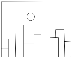
Fig. 11.1. A line drawing of a city.
