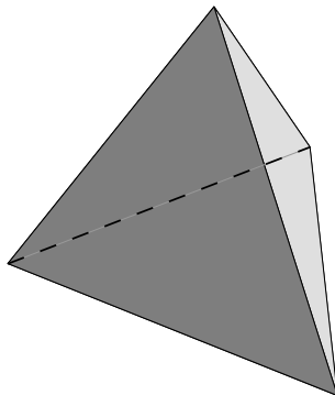
Fig. 15.57. A regular tetrahedron (see Exercise 37).
