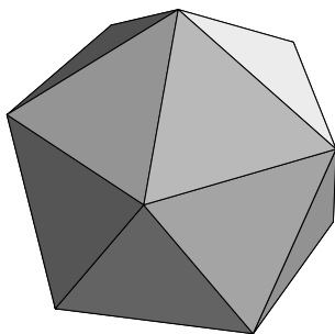
Fig. 15.59. An icosahedron.
