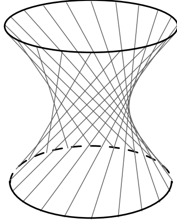
Fig. 15.24. The lines generating a hyperboloid of revolution of one sheet.
