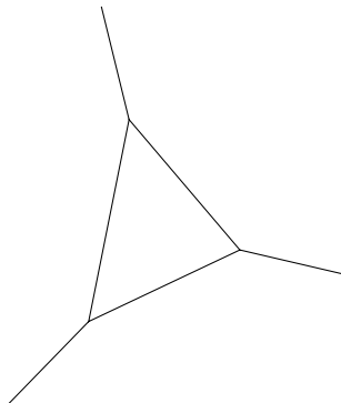
Fig. 15.55. A partitioning of the plane for Exercise 26(d).
