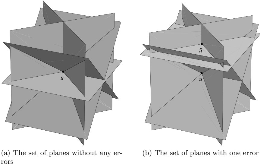
Fig. 6.4. The planes of system (6.12).
