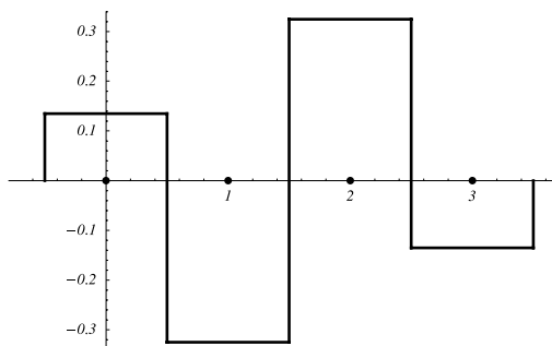
Fig. 12.10. The discrete function g of Exercise 4 (b).
