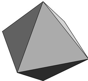
Fig. 15.58. An octahedron.
