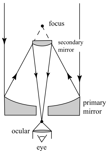
Fig. 15.14. Schmidt-Cassegrain telescope.
