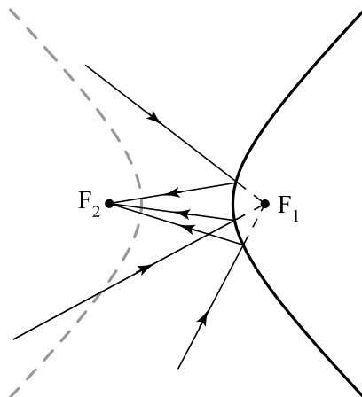
Fig. 15.19. A remarkable property of the hyperbola.
