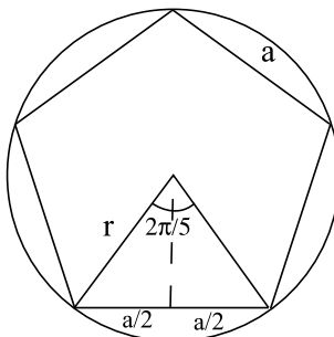
Fig. 15.44. Radius of the circle circumscribed about a regular pentagon.
