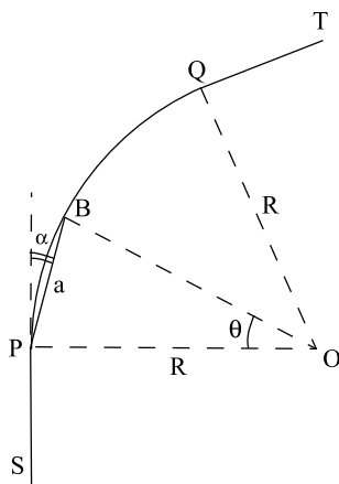
Fig. 15.46. Marking off a highway.
