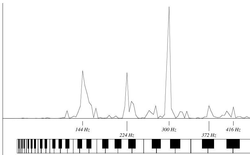
Fig. 10.8. The function e_k = k(C_k^2 + S_k^2) as a function of frequency (4k) Hz for frequencies below 450 Hz.
