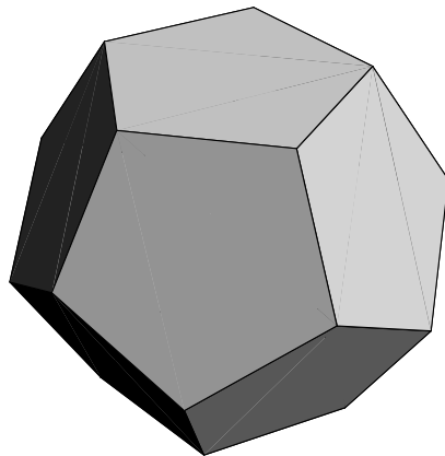
Fig. 15.41. A dodecahedron.
