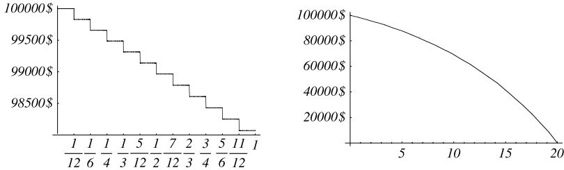
Fig. 5.2. Outstanding balance during the first year (left) and during the 20-year amortization period (right). See Example 5.2.
