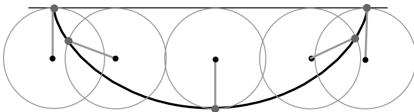
Fig. 14.4. Constructing a cycloid.
