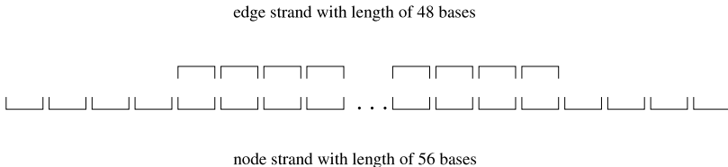
Fig. 13.2. Length of chain encoding paths.
