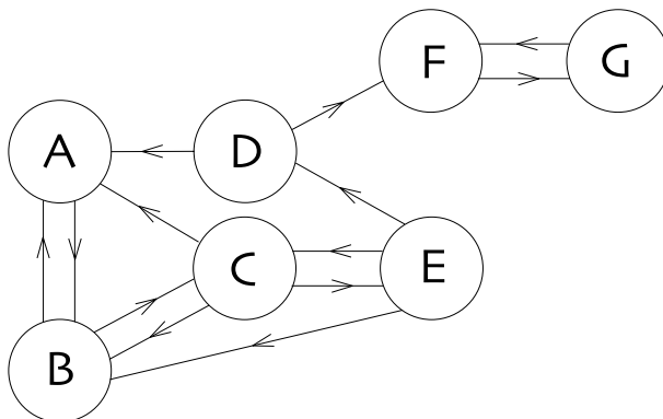
Fig. 9.4. A web of seven pages.
