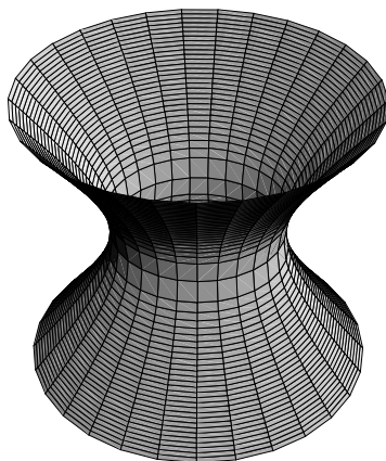
Fig. 15.21. A hyperboloid of revolution of one sheet.
