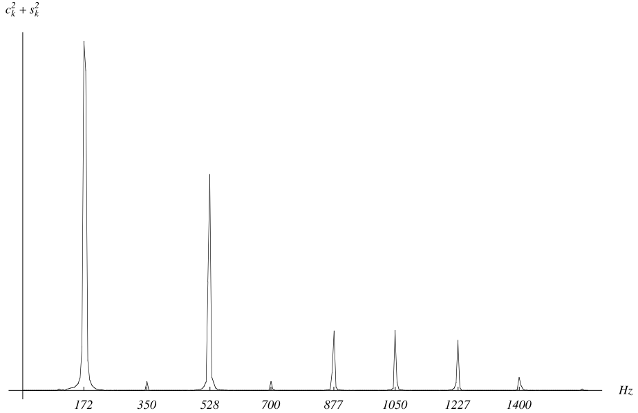
Fig. 10.14. The spectrum of the first note of Rhapsody in Blue . The frequencies of local maxima are indicated. (See Exercise 10.)
