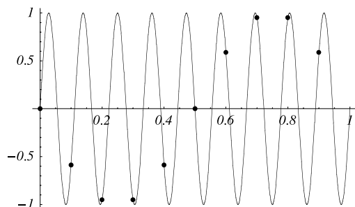
Fig. 10.15. A simple example of aliasing. (See Exercise 14.)
