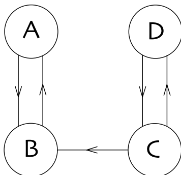
Fig. 9.7. The web of Exercise 5, with two pairs connected by a single link.
