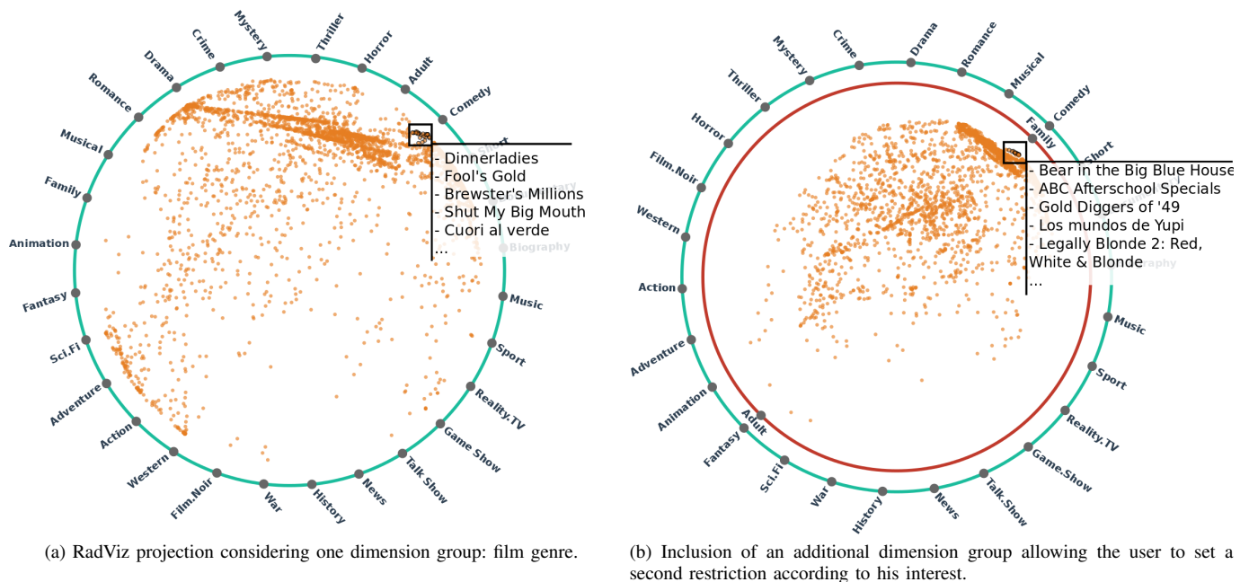
Fig. 6. Concentric RadViz with the IMDB-F film dataset.
