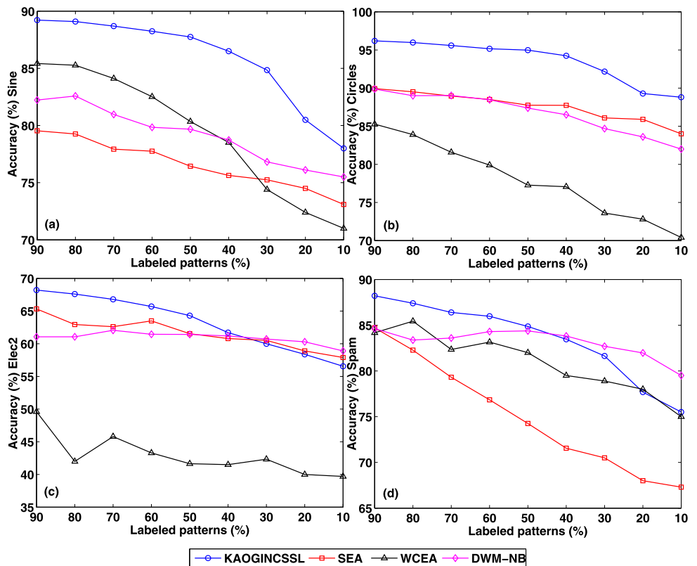
Fig. 4 Experiments with nine different percentages of labeled patterns in each data set for the domains Sine, Circle, Elec2 and Spam
