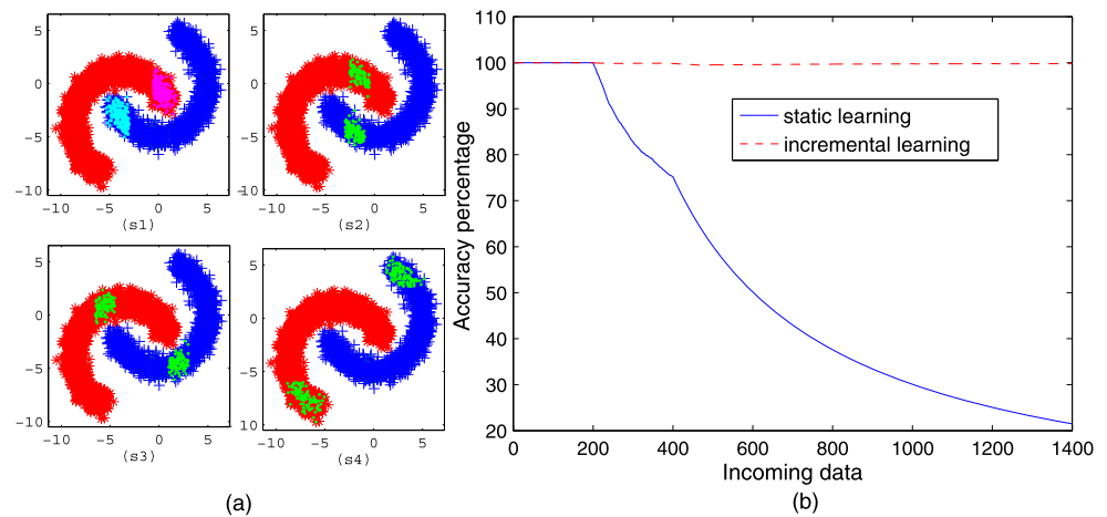
Fig. 2 (a) Artificial data set (Banana set) divided into sequential groups for simulating a non-stationary domain. The highlighted examples represent those chosen examples in a run. (b) Cumulated accuracy for static and incremental learning using the KAOG classifier
