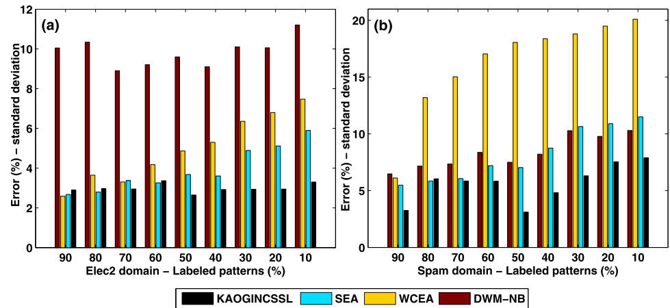
Fig. 5 Standard deviations for the four compared algorithms when processing the real domains (Elec2 and Spam) within the nine different percentage of labeled patterns in each data set
