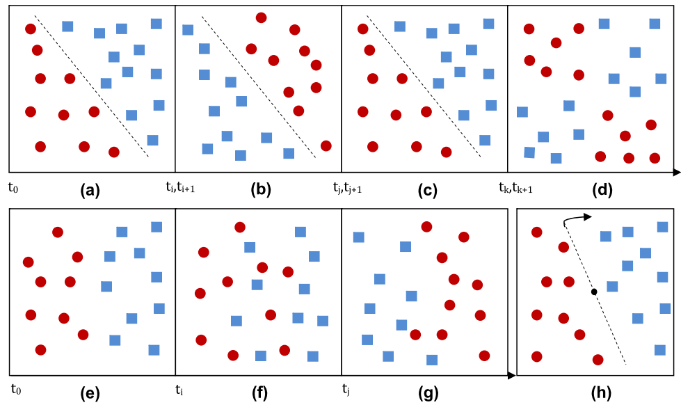
Fig. 1 Frequent concept drift characterizations, (a)–(d), abrupt drifts with recurrence; (e)–(g) gradual drift and (h) example subjugated to the velocity it is modified
