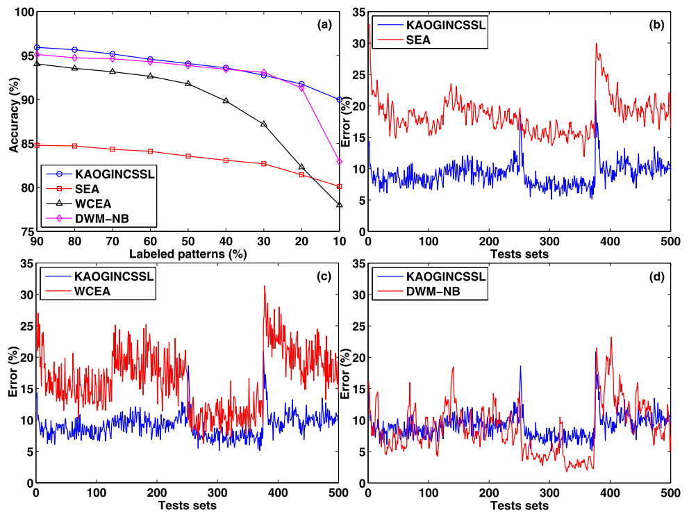
Fig. 3 Experiments with the SEA domain, (a) average accuracy for nine experiments with different percentages of labeled patterns, from 10 % to 90 %; and performance comparison through the SEA presentation with 20 % labeled patterns, between the KAOGINCSSL and (b) SEA, (c) WCEA and (d) DWM-NB
